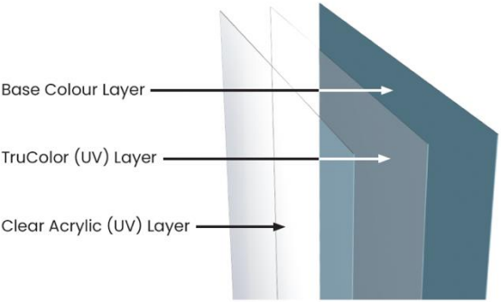
Above: TruColor features a unique three layer combination
